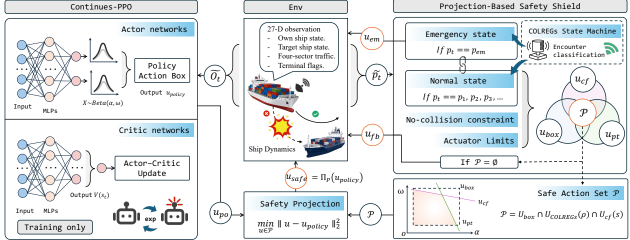
Figure 1 Overview of the method. A 27-dimensional observation enters the policy network, which emits a desired control command u_{\text{policy}} from a Beta distribution with bounded support. The rule state machine assigns the encounter to one of six situations. The safe control set U_{\text{safe}} is the intersection of the actuator limits, the half-plane of compliant directions, and the one-step collision-free constraint. A quadratic program projects u_{\text{policy}} onto u_{\text{safe}} , which is then passed to the environment. The projection is part of the environment transition, so the shield sits inside the training loop. The two bypasses are exclusive. An emergency situation goes straight to the emergency controller, and every other situation falls back only when U_{\text{safe}} is empty. The panel at the lower right sketches the three constraint sets in the control plane.
