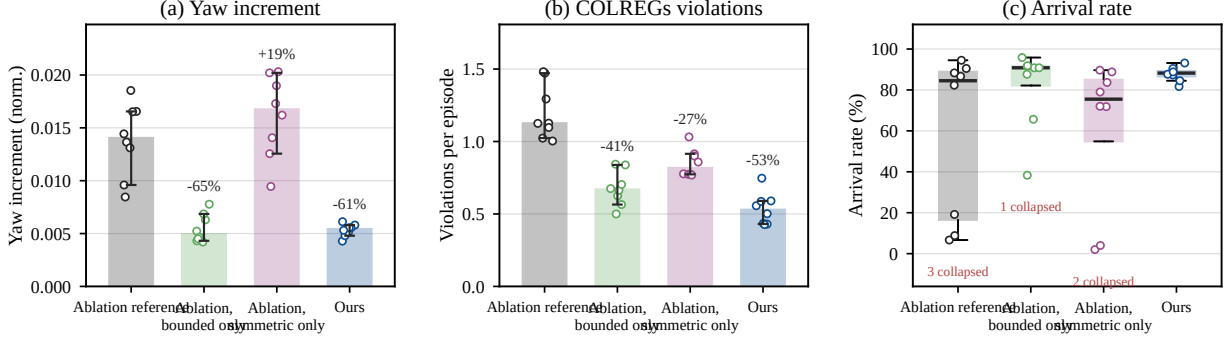
Figure 3 The 2 \times 2 ablation. Paired by seed. Bars are medians across seeds, error bars are bootstrap 95% intervals, and open points are single seeds. The label above each bar is the change relative to the leftmost bar. The paired tests are reported in the text. The arrival rate is bimodal, so it is drawn as a box plot and the number of diverged seeds is printed below each box.
