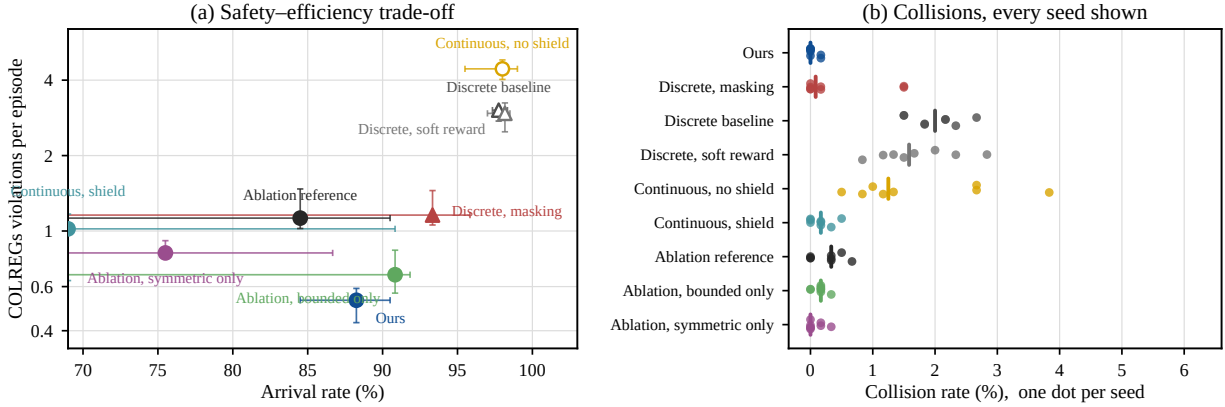
Figure 2 Safety and efficiency. Official test set, the same source as Table 3. Points are medians across seeds and error bars are bootstrap 95% intervals resampled over seeds. Circles are continuous action spaces, triangles are discrete ones, and filled markers carry a shield. The lower right of panel (a) is the ideal region. The bars are wide because several configurations contain a diverged seed.
