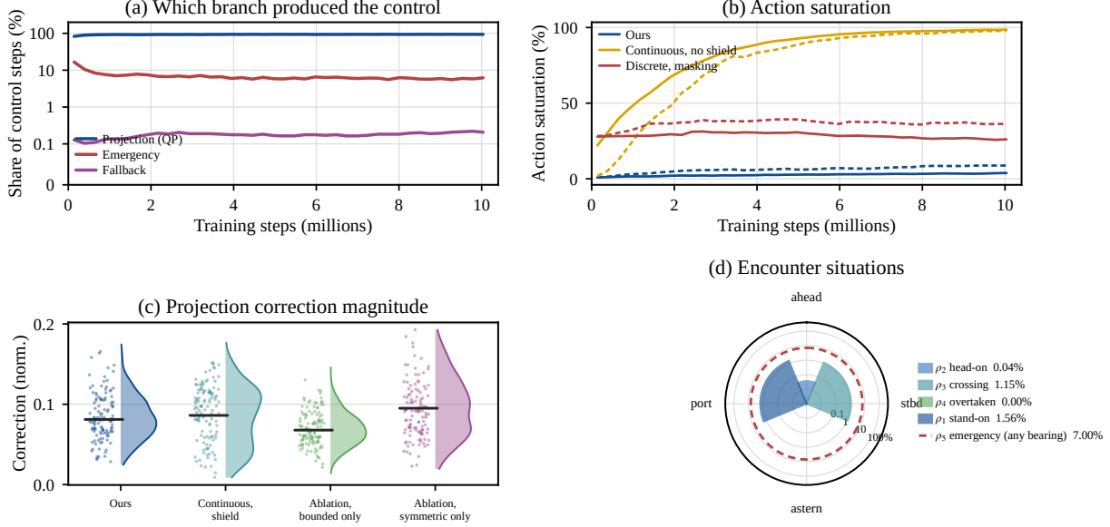
Figure 5 Behavior of the shield. In panel (d) the angle is the sector in which the convention defines each situation, not the measured bearing distribution of target vessels, and the radius is logarithmic. This figure is collected during training rather than at evaluation.
