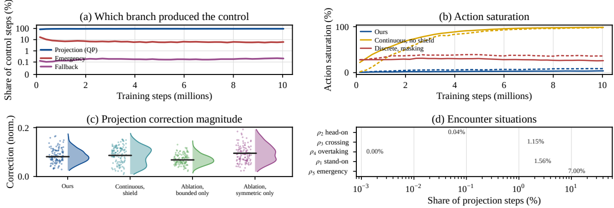
Figure 5 Behavior of the shield. Panel (d) is the share of projection steps in each situation, on a logarithmic scale. This figure is collected during training rather than at evaluation.
