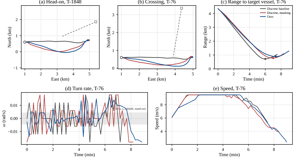
Figure 6 Tracks of three configurations in two encounters. Scenarios are picked by geometry alone and never by outcome: for each encounter situation, the smallest closest approach under constant velocity, which is 7 m for T-1848 and 2 m for T-76. The seed is s_0 and the checkpoint is the last one of the run rather than the one selected on the validation set. The open circle and the square mark the start of the own vessel and of the target vessel, and the dashed line is the recorded track of the target vessel. In (c) the dot marks the closest approach reached by each configuration and the dashed line is the closest approach under constant velocity. Panels (d) and (e) give the turn rate and the speed of the own vessel over the same encounter, recovered from the recorded states. The shaded band in (d) is the stand-on tolerance used by the shield; the offline scorer counts a violation from the heading change accumulated over an obligation period, which is a different test (Section 5.2).
