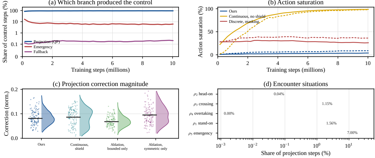
Figure 4 Behavior of the shield. Panel (d) is the share of projection steps in each situation, on a logarithmic scale. This figure is collected during training rather than at evaluation.
