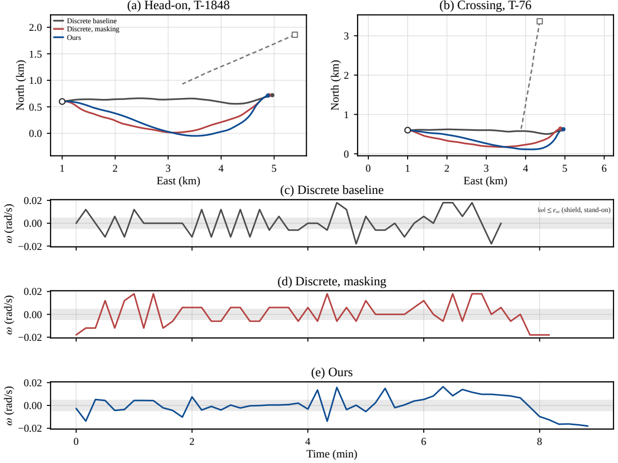
Figure 5 Tracks and turn rate in two encounters. Scenarios are picked by geometry alone: the smallest constant-velocity closest approach of each situation, 7 m for T-1848 and 2 m for T-76. Seed s_0 , at the last checkpoint rather than the one selected on the validation set. In (a) and (b) the circle and the square are the starts of the own and the target vessel, and the dashed line is the recorded target track. Panels (c) to (e) share one turn-rate scale and come from the crossing encounter. The shaded band is the stand-on tolerance of the shield, and the offline scorer applies a different test (Section 5.2).
