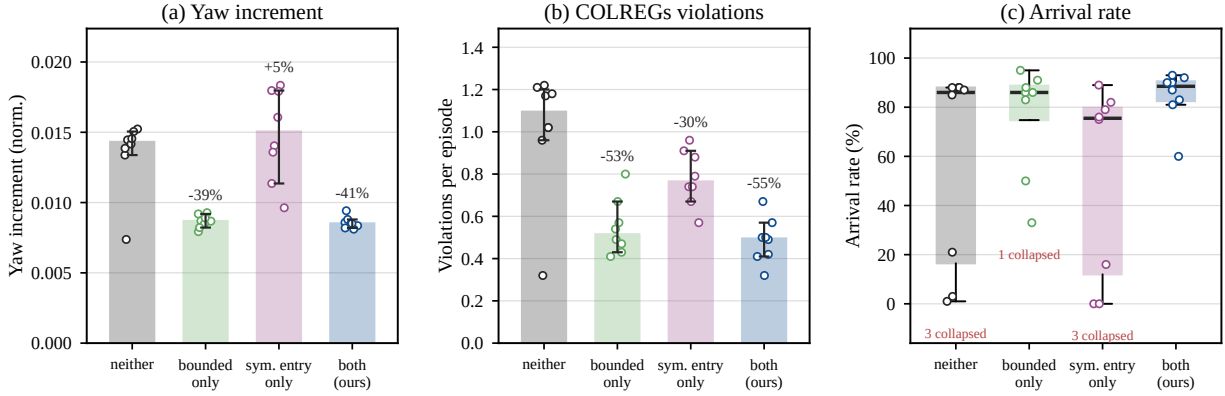
Figure 2 The 2 \times 2 ablation, paired by seed. (a) and (b) Bars are medians across seeds and error bars are bootstrap 95% intervals resampled over seeds. Above each bar are the change relative to the leftmost bar, the mark of the paired signed-rank test, and the number of seeds that moved in the same direction. (c) Box plot of the arrival rate, with the number of diverged seeds below each box and open points for single seeds. Provisional: values are from the validation set.
