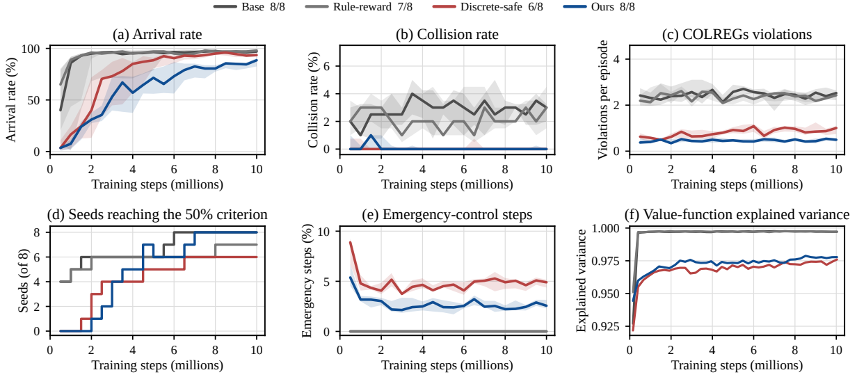
Figure 3 Sample efficiency and training reliability against training steps. Thick lines are medians and shaded bands are interquartile ranges, both over converged seeds only. The legend gives the number of converged seeds out of 8. The axis starts at the first evaluation point. (a) Arrival rate. (b) Collision rate. (c) COLREGs violations per episode. (d) Seeds that meet the convergence rule, counted over all 8. (e) Share of steps under emergency control. (f) Explained variance of the value function. Provisional: values are from the validation set.
