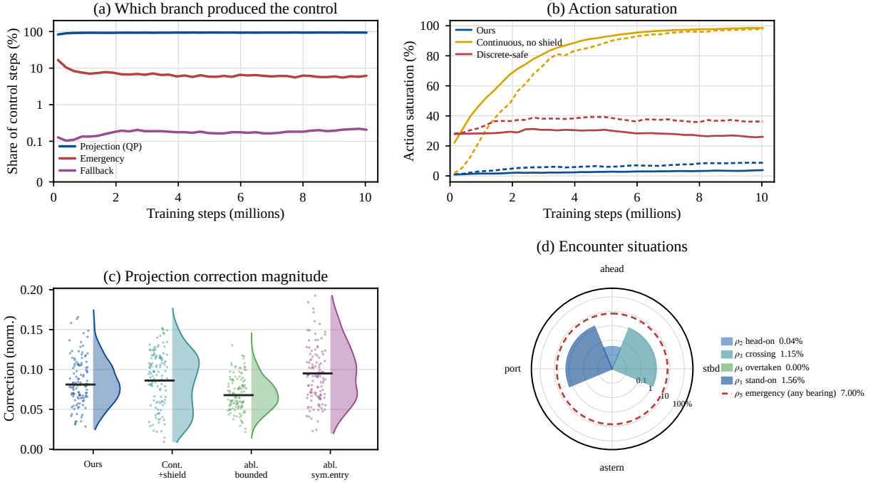
Figure 4 Behavior of the shield during training. (a) Which branch produced each control command, on a logarithmic axis. (b) Saturation of the action, with the turn axis solid and the acceleration axis dashed. (c) Distribution of the size of the projection correction, with single samples on the left half, a kernel density on the right half, and the median as a black line. (d) Share of each encounter situation, on a logarithmic radius. The angle is the sector in which the convention defines the situation, not a measured bearing distribution. The emergency situation belongs to no sector and is drawn as a dashed ring. Values are collected during training.
