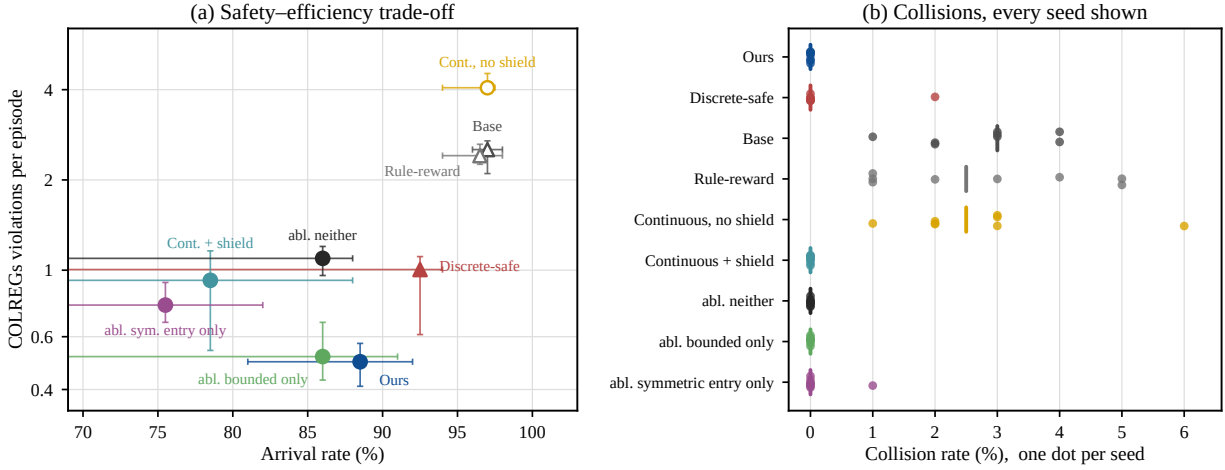
Figure 1 Safety and efficiency. (a) Arrival rate against COLREGs violations per episode, on a logarithmic axis. Points are medians across seeds and bars are bootstrap 95% intervals resampled over seeds. Circles are continuous action spaces, triangles are discrete ones, and filled markers carry a shield. (b) Collision rate, one point per seed, with a bar at the median. Provisional: values are from the validation set.
