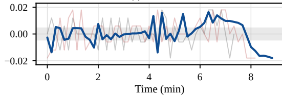
(f) Turn rate
