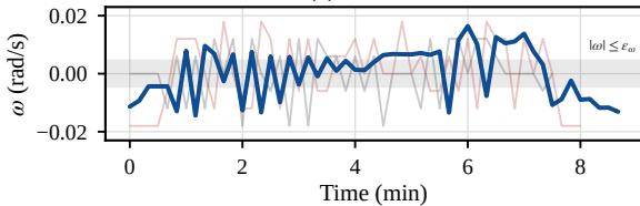
(e) Turn rate
