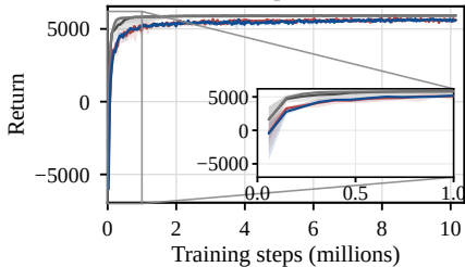
(a) Mean episode return
