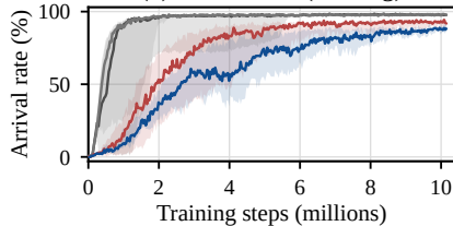
(b) Arrival rate (training)
