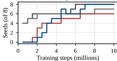
(e) Seeds reaching the 50% criterion
