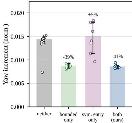
(a) Yaw increment
