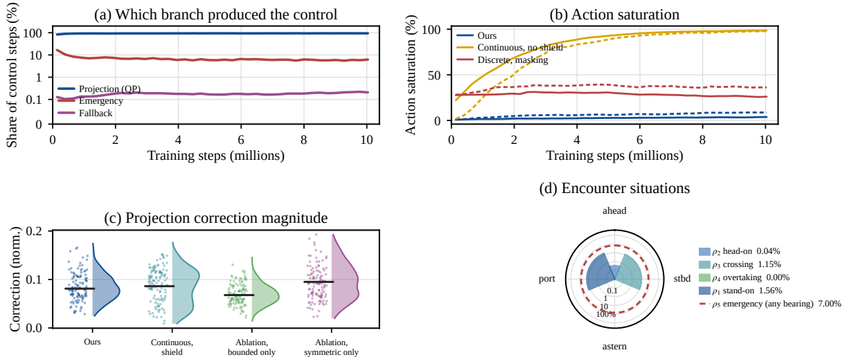
Figure 5 Behavior of the shield. In panel (d) the angle is the sector in which the convention defines each situation, not the measured bearing distribution of target vessels, and the radius is logarithmic. This figure is collected during training rather than at evaluation.
