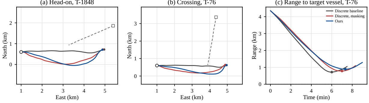
Figure 6 Tracks of three configurations in two encounters. Scenarios are picked by geometry alone and never by outcome. For each encounter situation the scenario was selected by the smallest closest approach under constant velocity. That distance is 7 m for T-1848 and 2 m for T-76. The seed is s_0 , one of the three declared in advance, and the checkpoint is the last one of the run rather than the one selected on the validation set. The open circle marks the start of the own vessel. The square marks the start of the target vessel. The dashed line shows the recorded track of the target vessel. In (c) the dot marks the closest approach reached by each configuration and the dashed line is the closest approach under constant velocity. This figure is a qualitative illustration and carries no quantitative claim.
