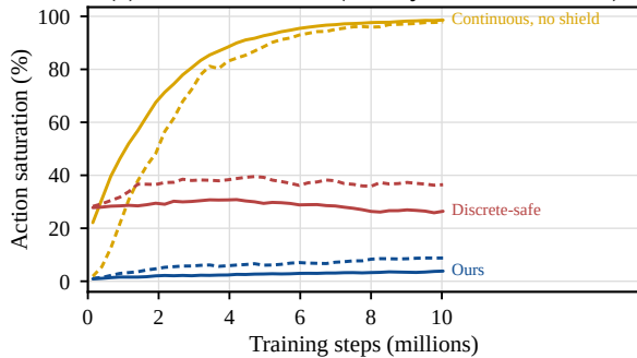
(b) Action saturation (solid: yaw, dashed: accel.)
