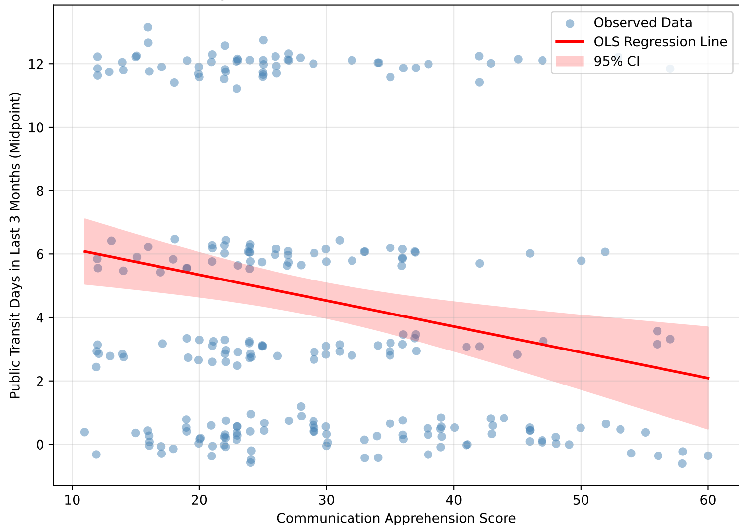
OLS Regression with Jittered Points and Confidence Interval
