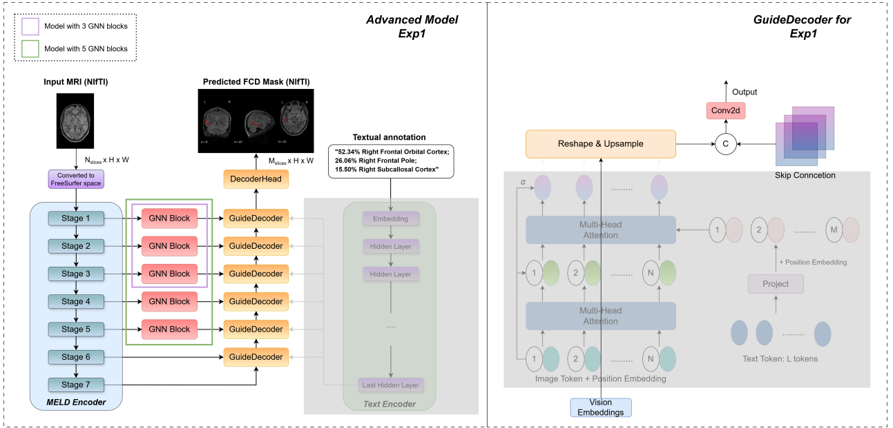
Figure 5.12: Architecture of Advanced Exp1: MELD surface-based features are extracted through a multi-stage GNN encoder (3- or 5-block variants) and passed through a hierarchical GuideDecoder with cross-attention to text embeddings. At each decoder stage, visual features are fused with text embeddings, reshaped, and upsampled through geometry-aware operations, before producing the final segmentation via the DecoderHead. The right panel illustrates the internal structure of the GuideDecoder layer, including self- and cross-attention over text and vision tokens, skip connections, and spatial upsampling.
