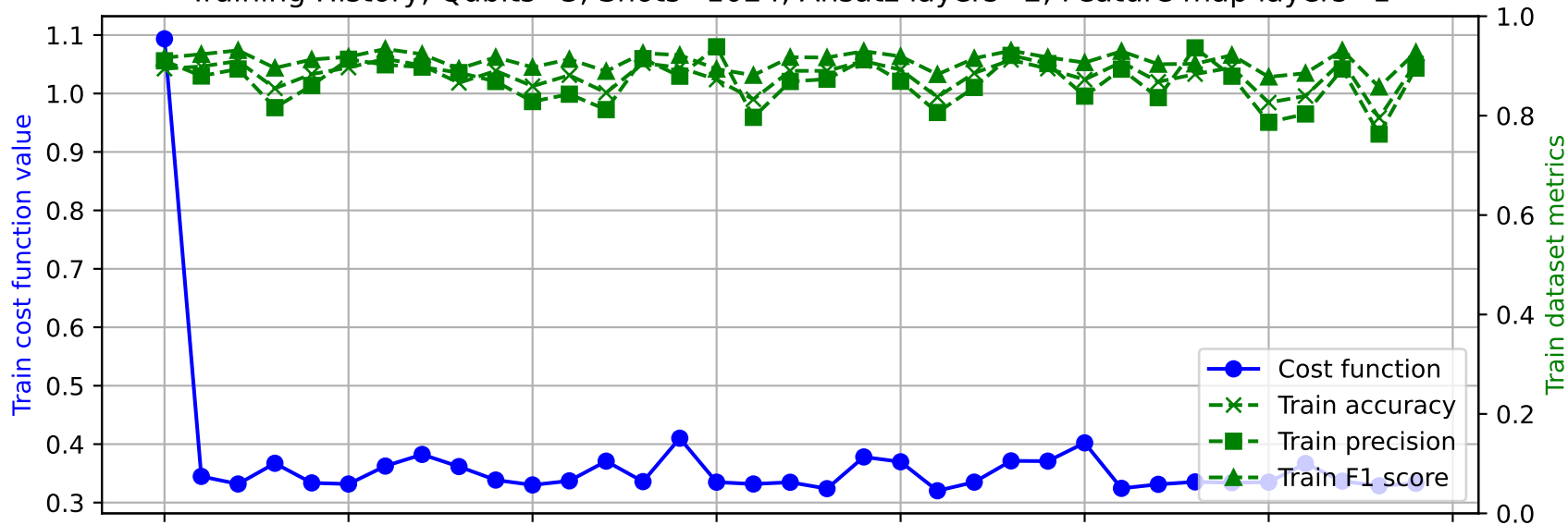
Training History, Qubits=3, Shots=1024, Ansatz layers=2, Feature map layers=1
