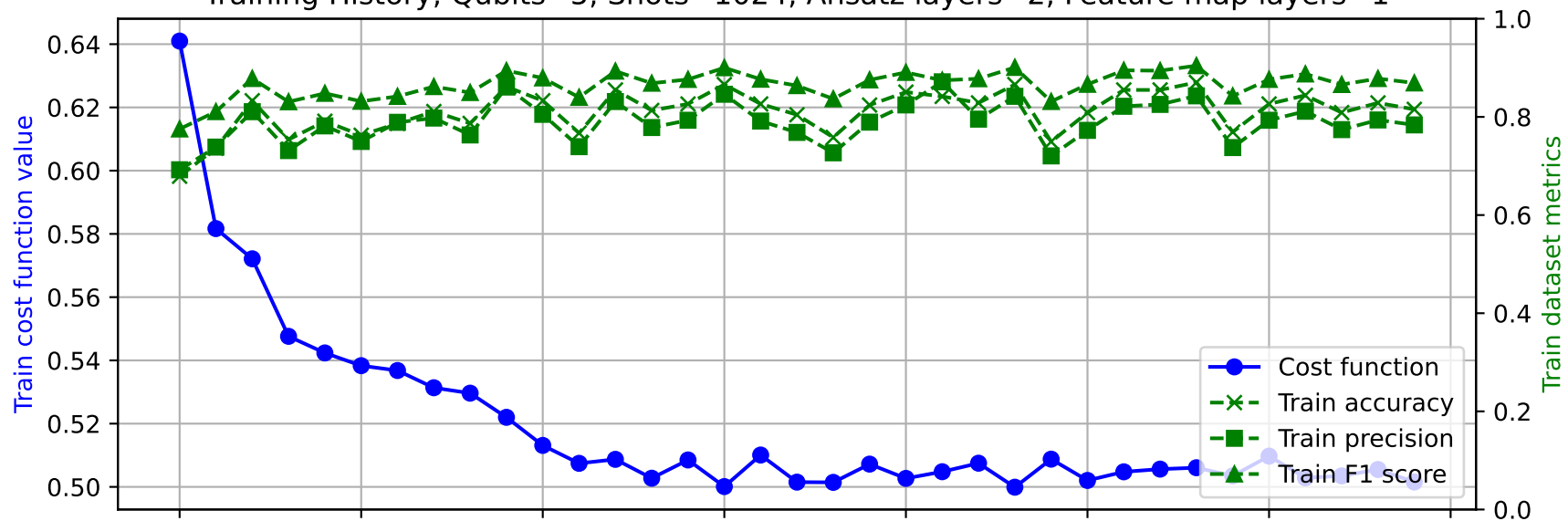
Training History, Qubits=5, Shots=1024, Ansatz layers=2, Feature map layers=1
