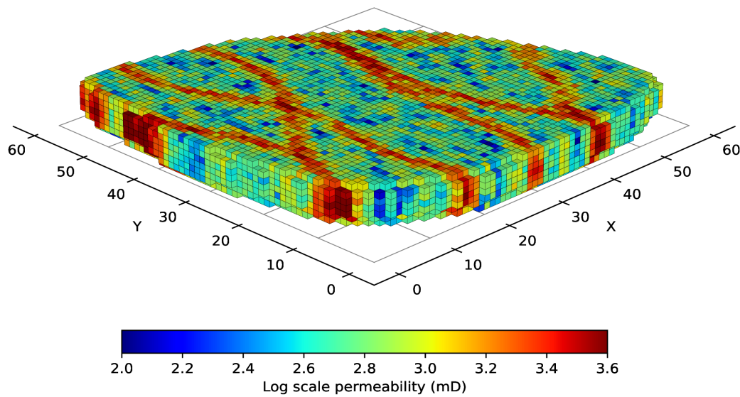
Figura 2.7: 3D Egg model
