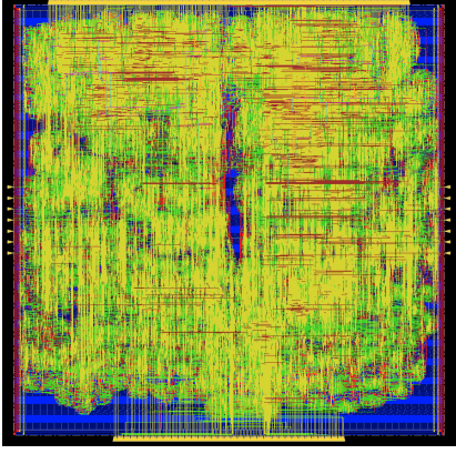
Fig. 16: Sparsity-Aware Attention Dual-Core Layout.
