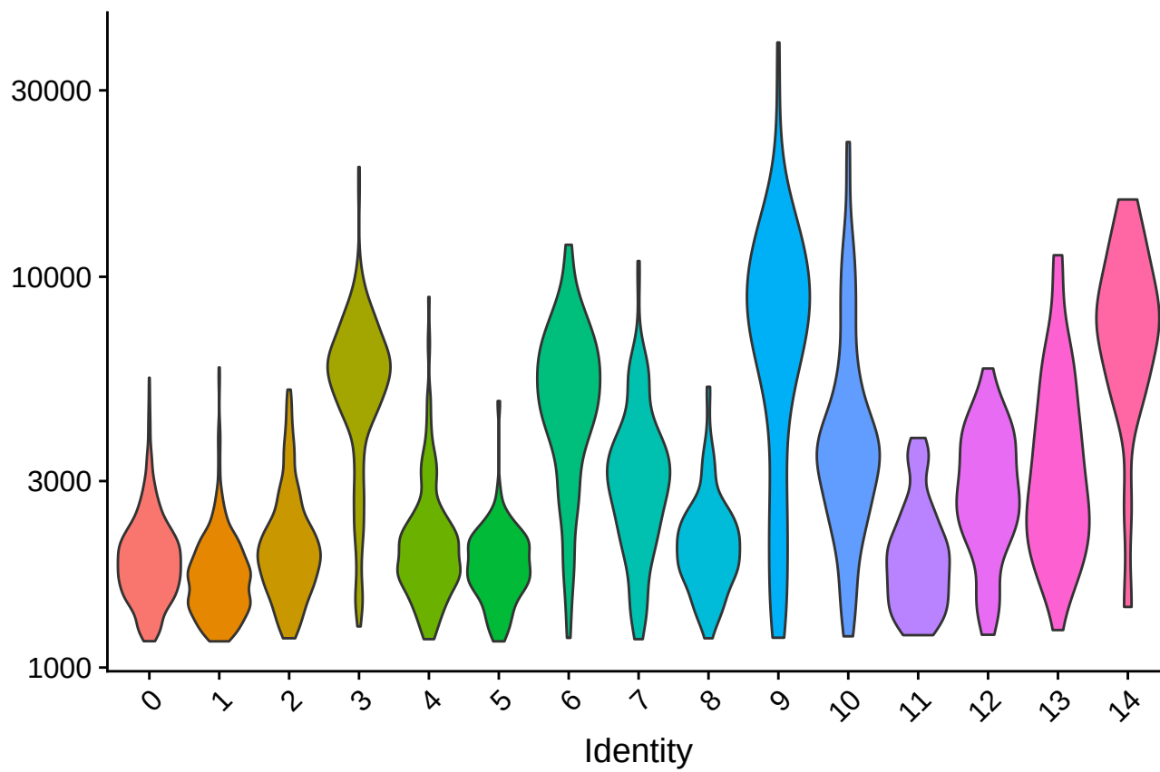
nCount_RNA
