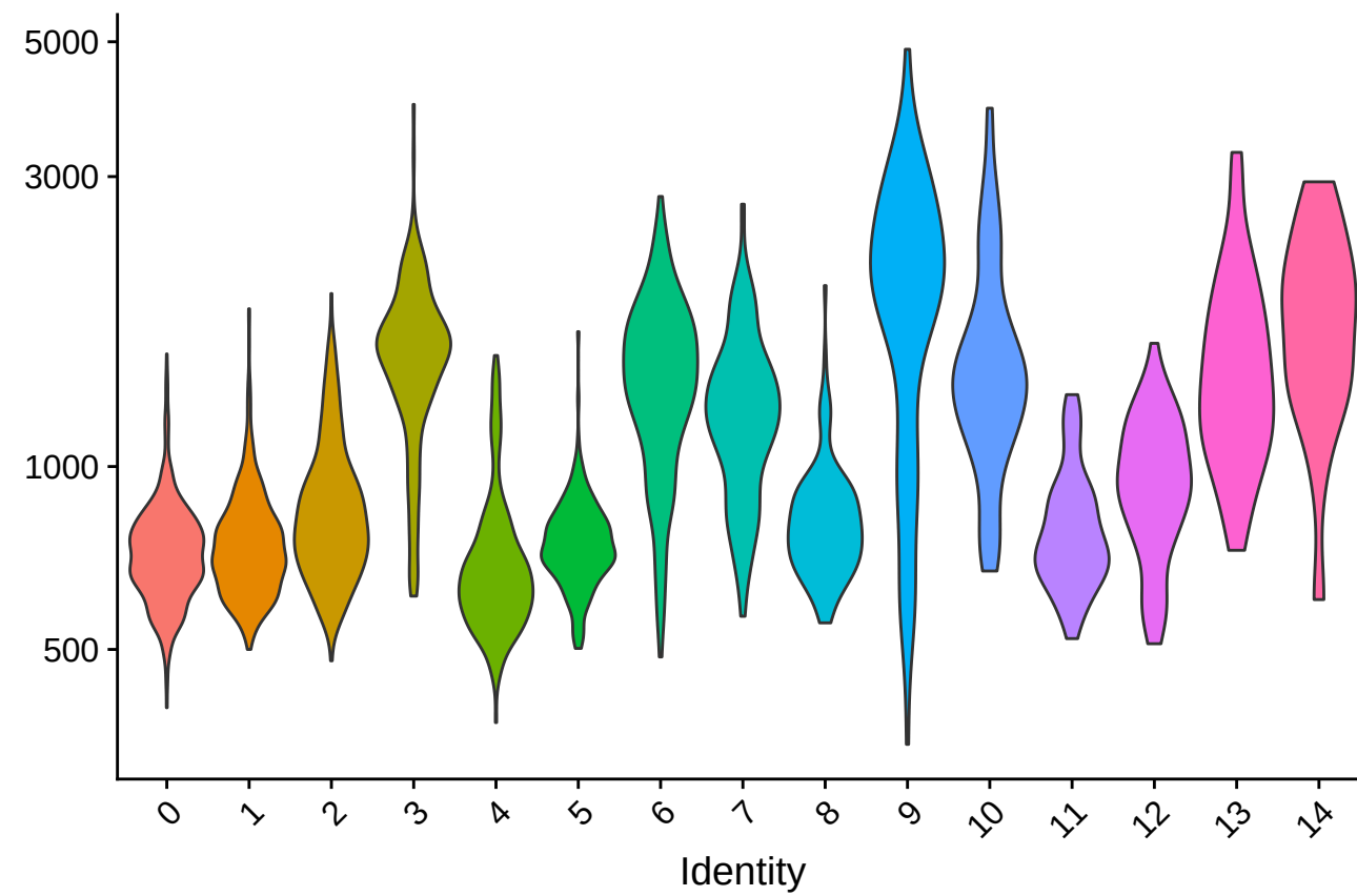
nFeature_RNA
