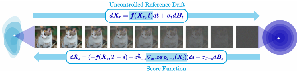
圖: Score-based 擴散模型。圖源: Figure 7 [T26]。
