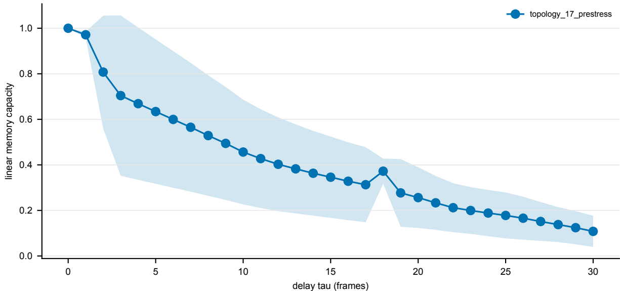
Fixed delayed-input linear memory capacity
