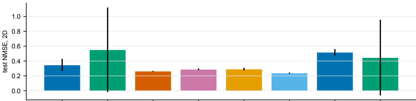
Input-history basis fit to hidden-node target; lower is better
