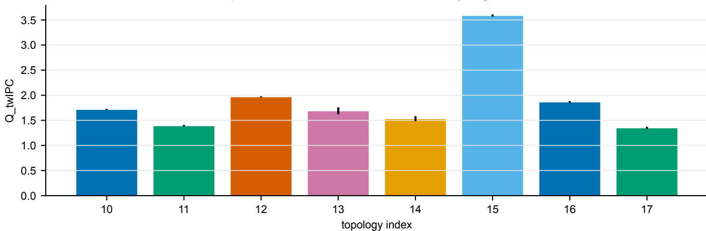
Task-specific IPC on fixed H=1, D=1 dictionary; higher is better
