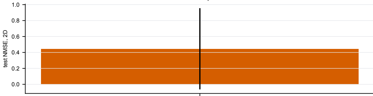
Task-specific IPC
