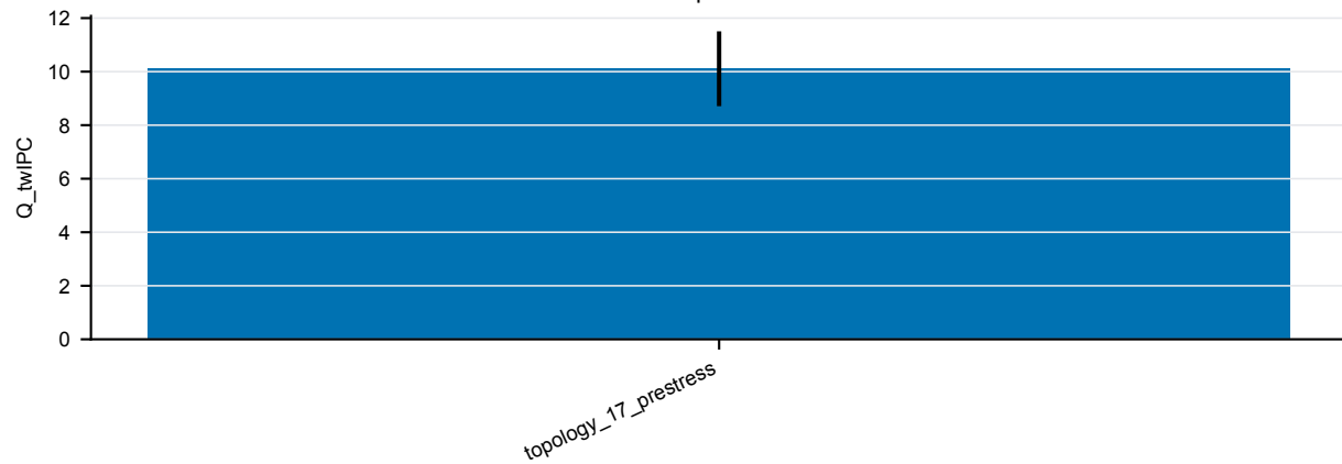
Task-specific IPC
