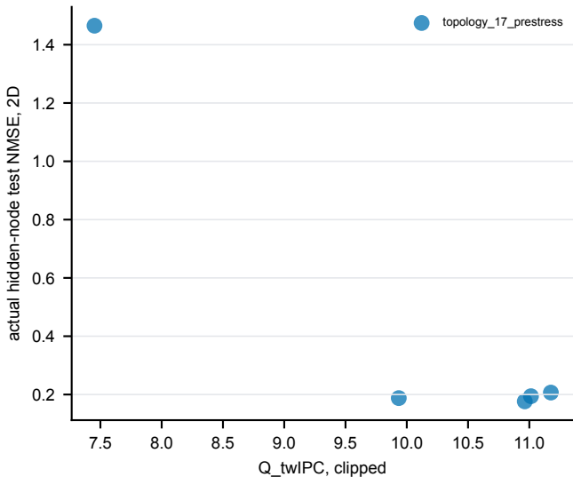
Task-specific IPC versus task error
