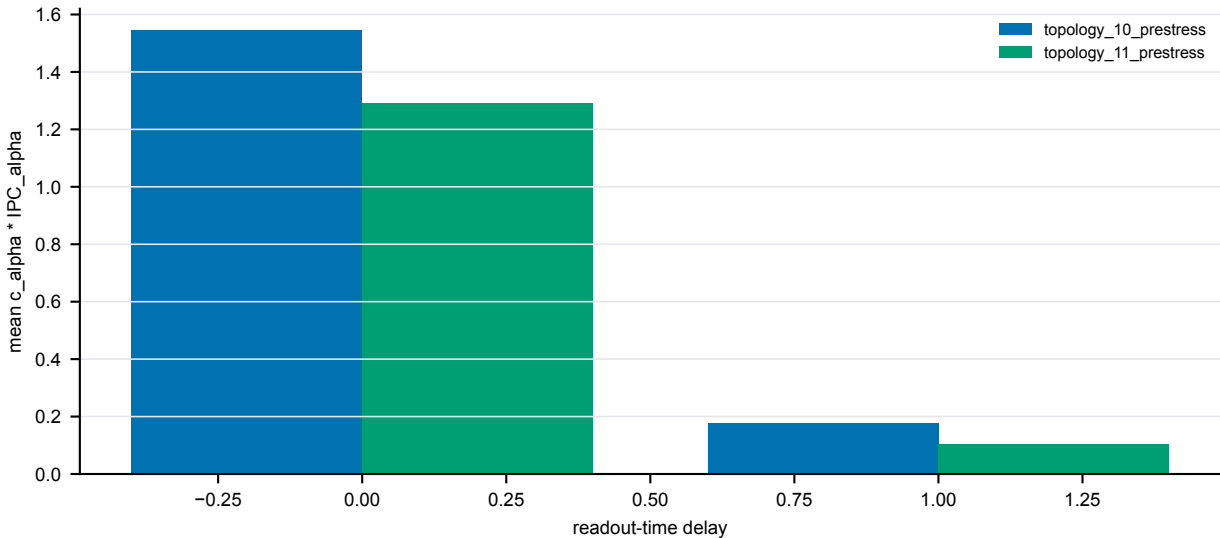
Delay-resolved task-specific IPC contribution
