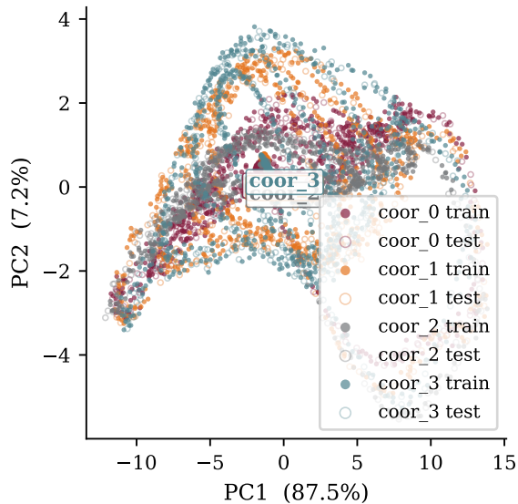
PC1 vs PC2 (filled=train, hollow=test)
