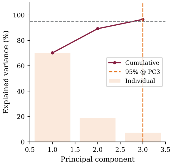
Scree plot
