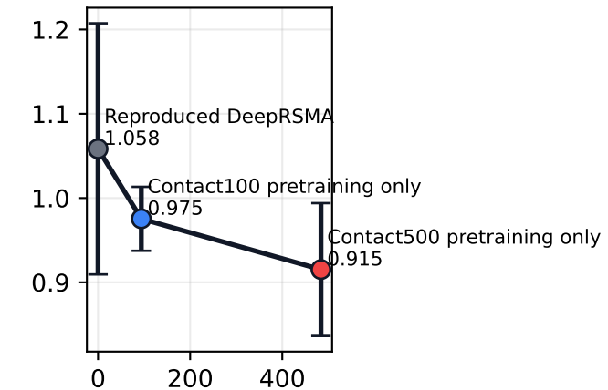
RMSE
