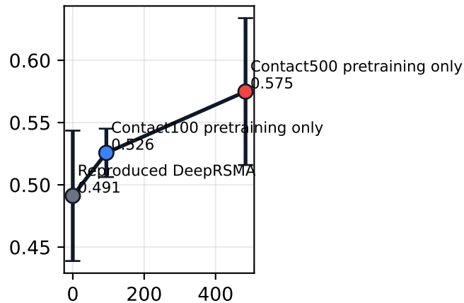
SCC
