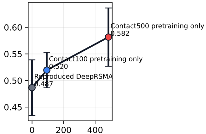
PCC
