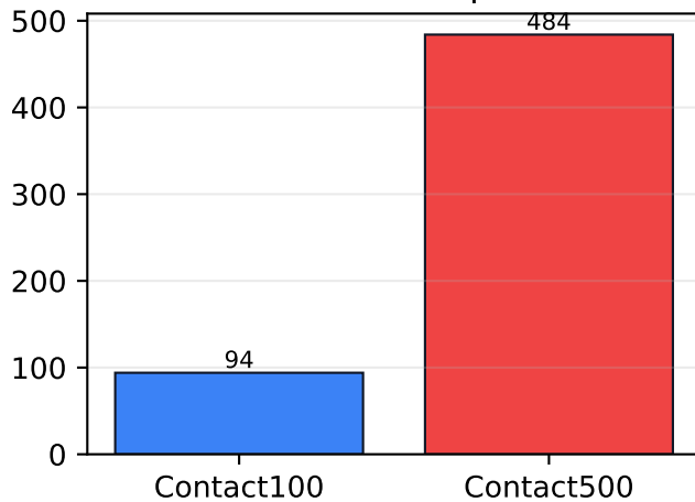
Positive contacts
