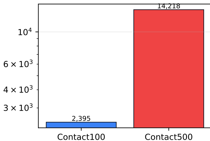
Positive contacts
