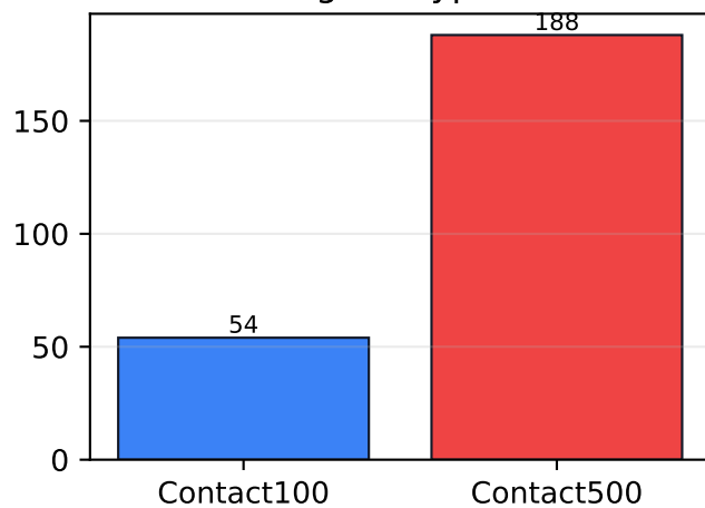
Nucleotide-atom pairs
