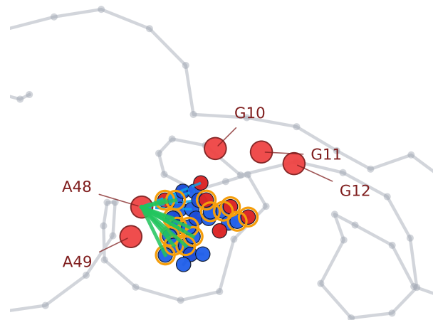
B. Binding pocket with top-k predictions
