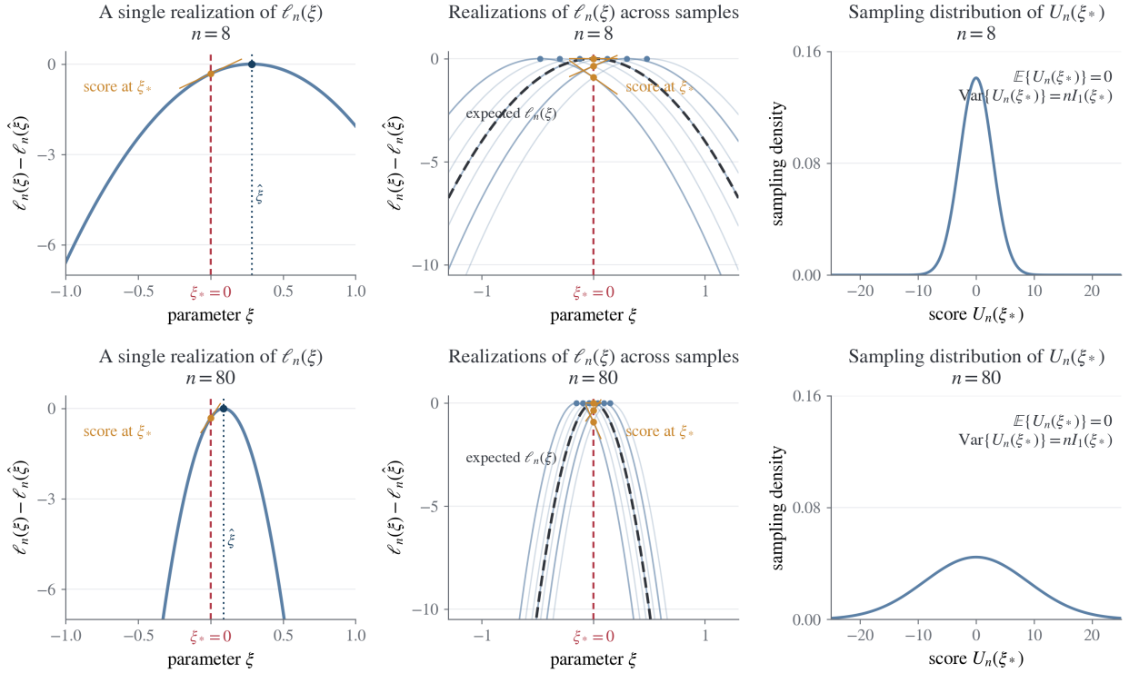
Figure 1: Score, likelihood curvature, and Fisher information under repeated sampling for a single-parameter model. (1) For a regular interior maximum, the MLE \hat{\xi} is obtained by setting the score U_n(\xi) := \ell'_n(\xi) to zero. The left column shows one realization of the log-likelihood, while the middle column shows repeated realizations from independent samples of size n . The yellow tangent lines and points represent the scores U_n(\xi_*) , i.e., the slopes of the realized log-likelihoods at the true parameter \xi_* , which fluctuate from sample to sample. (2) Comparing the top and bottom rows, increasing n makes the log-likelihood more sharply curved downward, so the observed negative curvature -\ell''_n(\hat{\xi}) becomes larger in magnitude. At the same time, the total score U_n(\xi_*) , being the sum of n individual scores, exhibits greater variability across repeated samples (right column). This larger score variance reflects more Fisher information (rather than greater uncertainty about \xi ) and yields a more concentrated MLE, since the steeper curvature converts a given score perturbation into a smaller displacement of \hat{\xi} . (3) The Bartlett identities formalize this relationship. First, \mathbb{E}_{\xi_*}[U_n(\xi_*)] = 0 , so the score at true \xi_* has mean zero. Moreover, \mathbb{E}_{\xi_*}[-\ell''_n(\xi_*)] = \text{Var}_{\xi_*}[U_n(\xi_*)] = \mathbb{E}_{\xi_*}[U_n(\xi_*)^2] \stackrel{\text{def}}{=} I_n(\xi_*) , that is, the expected negative log-likelihood curvature and the score variance are equivalent measures of Fisher information: more observations imply larger curvature, greater score variance, and a more concentrated MLE (i.e., a smaller asymptotic variance). The precise relationships are developed in the following subsections.
