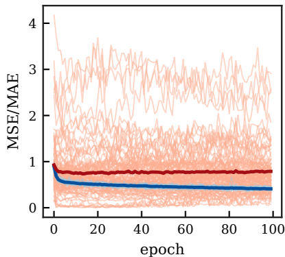
GNN (slope=-8e-04)
