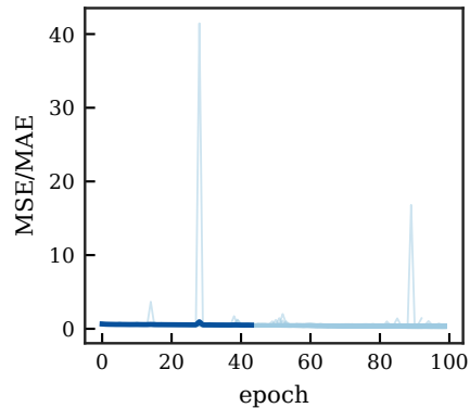
ST-GNN (slope=-1e-03)
