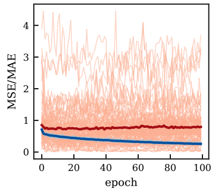
ST-GNN (slope=-1e-03)
