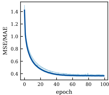
GNN (slope=-8e-04)
