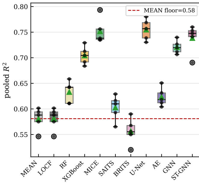
profile (points = 5 seeds)
