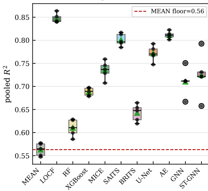
blackout (points = 5 seeds)
