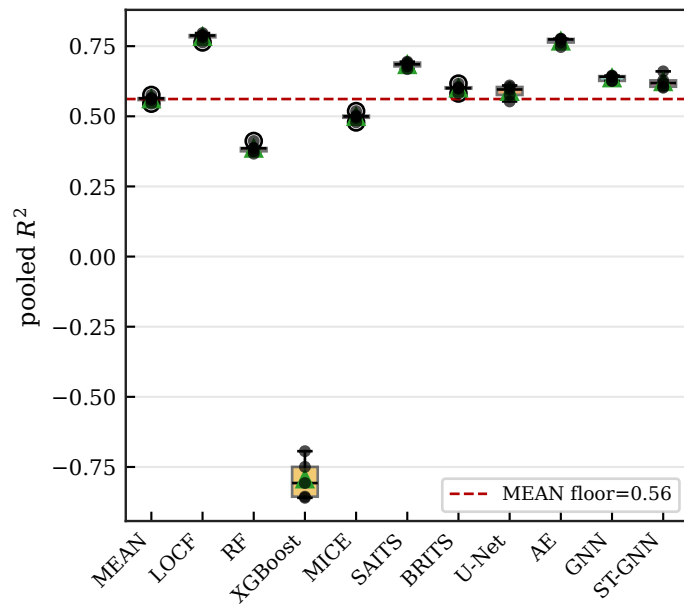
blackout (points = 5 seeds)
