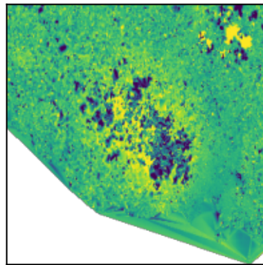
CNN-TCN hybrid
