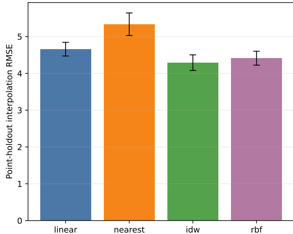
Interpolation-only accuracy
