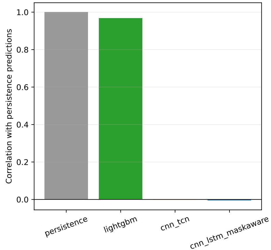
Persistence similarity
