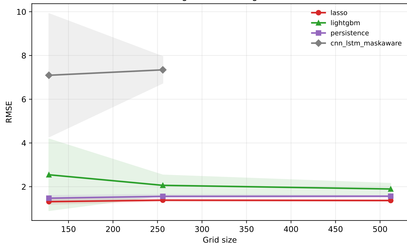
Resolution scaling under the original CAGEO suite
