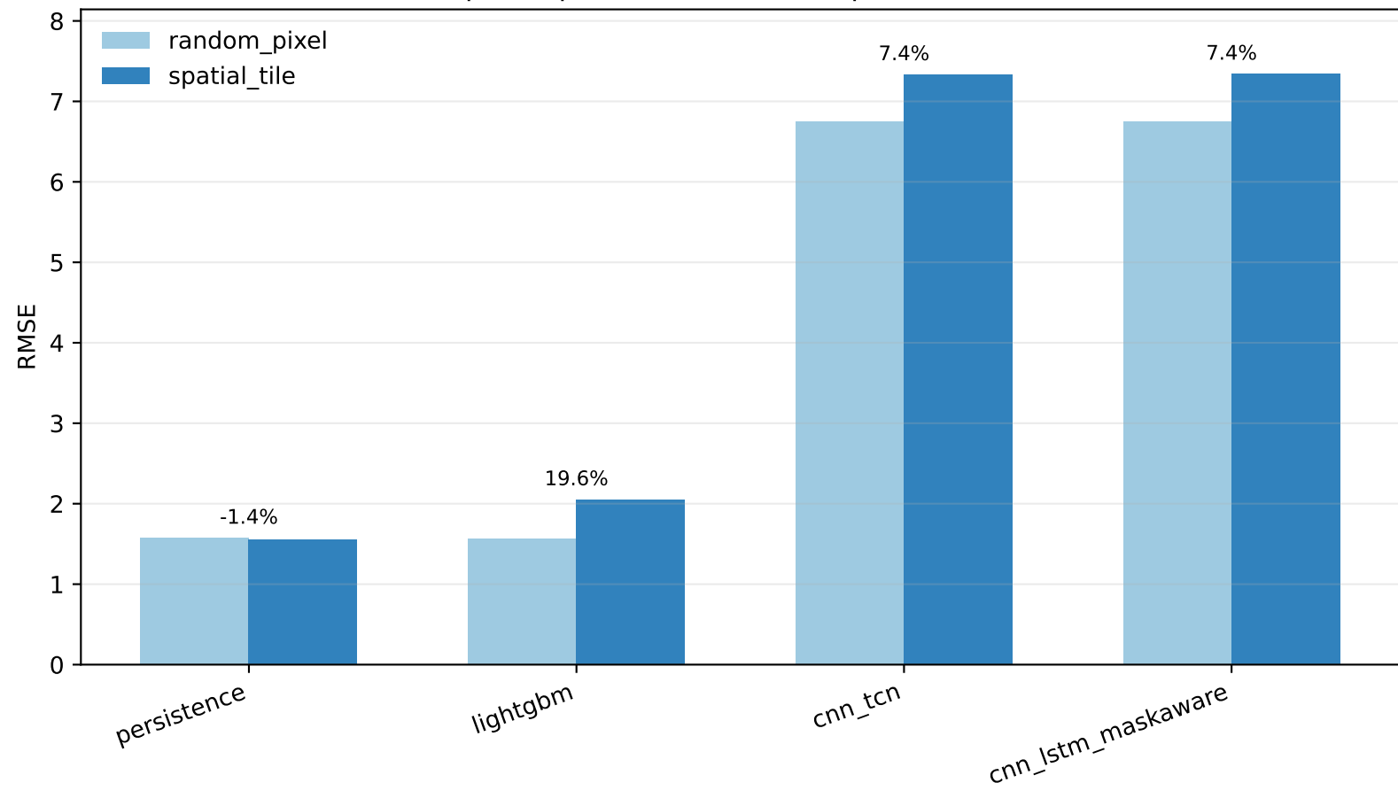
Random-pixel optimism relative to spatial-tile evaluation
