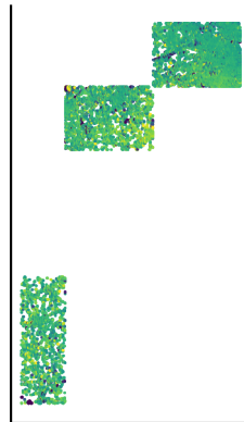
Absolute-error reduction
