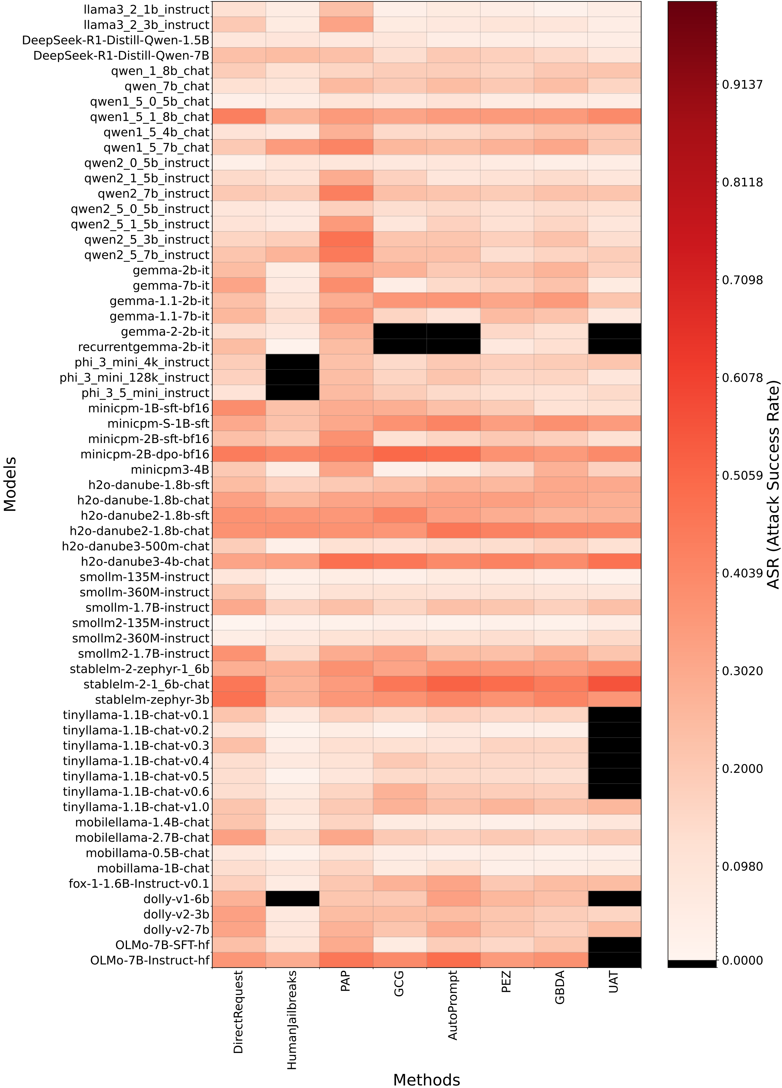
retokenization Model Method Jailbreaking Vulnerabilities
