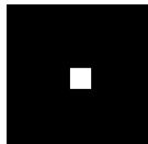
g_2 : Quadratic
