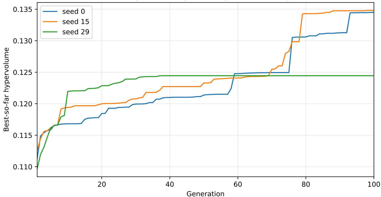
Stage 2 convergence diagnostic: xerces-j
