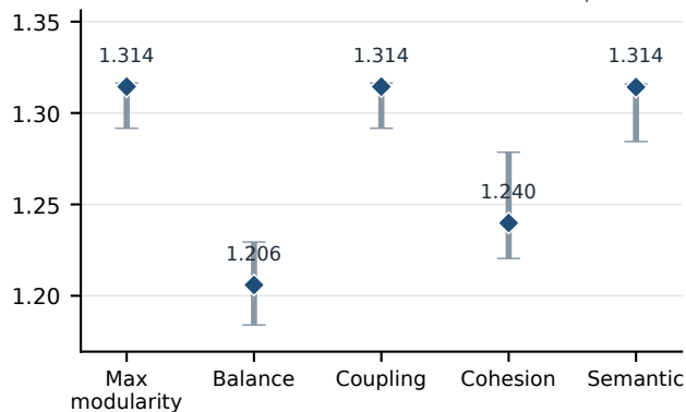
(a) Imbalance
