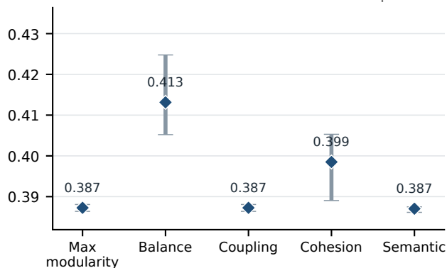
(c) f_{\text{sem}}
