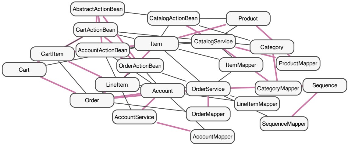
(a) Structural evidence 53 edges: 28 structural-only and 25 overlap
