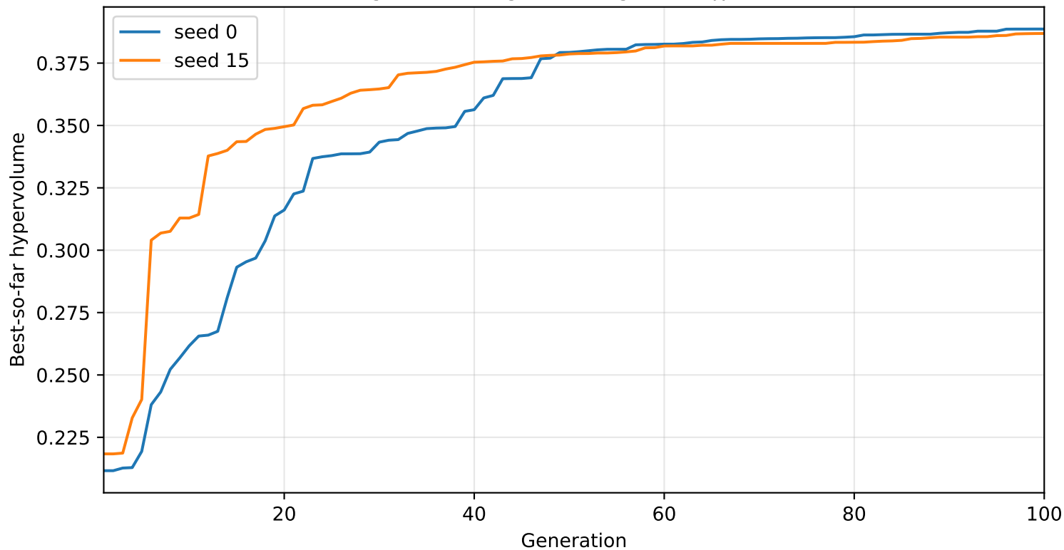
Stage 2 convergence diagnostic: jpetstore
