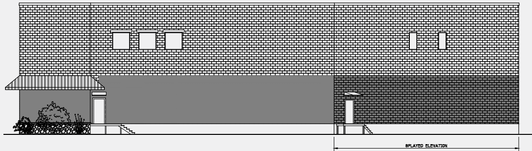
1 REAR ELEVATION SCALE 1/8" = 1'-0"
