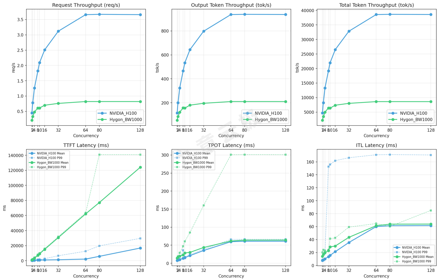
MiniMax-M2.5 Performance Trends by Concurrency
