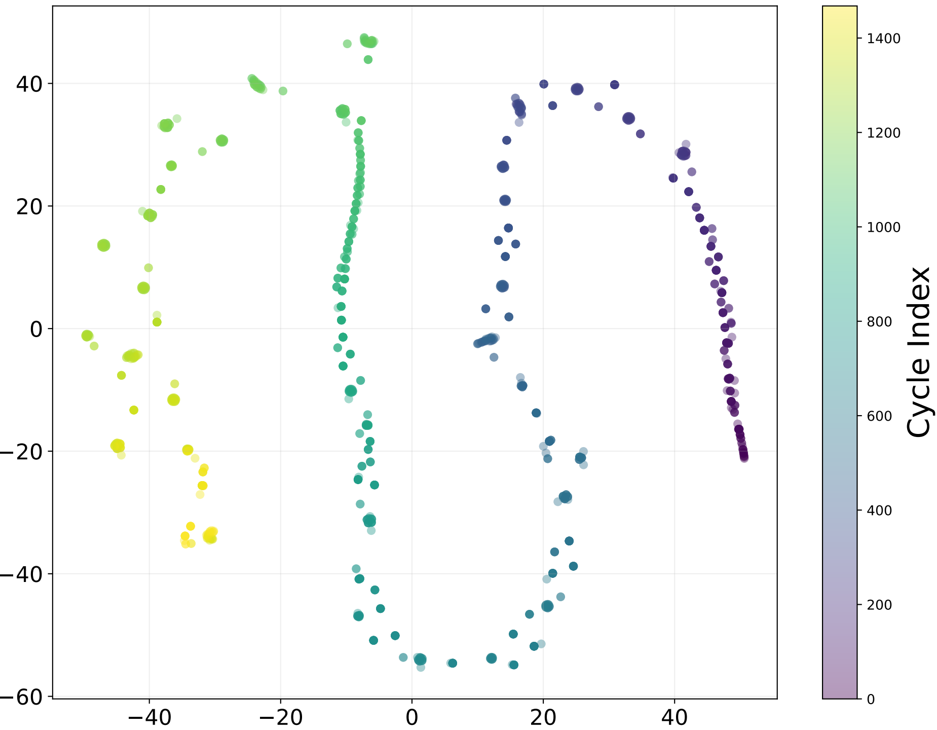
Manual Features
