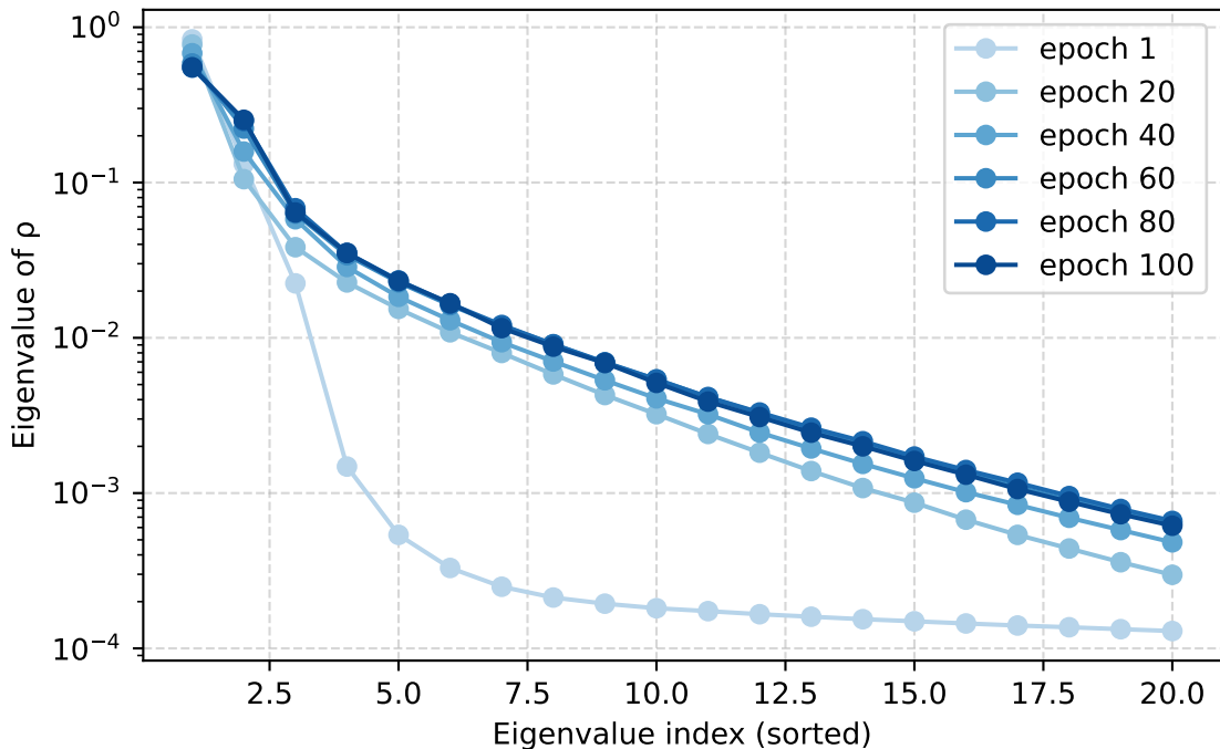
Top-20 eigenvalues of \rho at selected epochs
