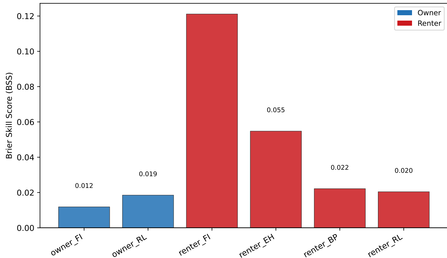
Brier Skill Score — Post-Calibration (validation set)
