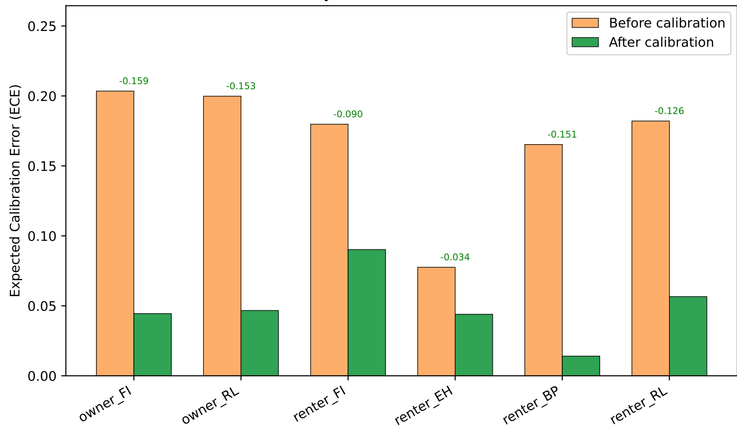
Calibration Improvement: ECE Before vs After
